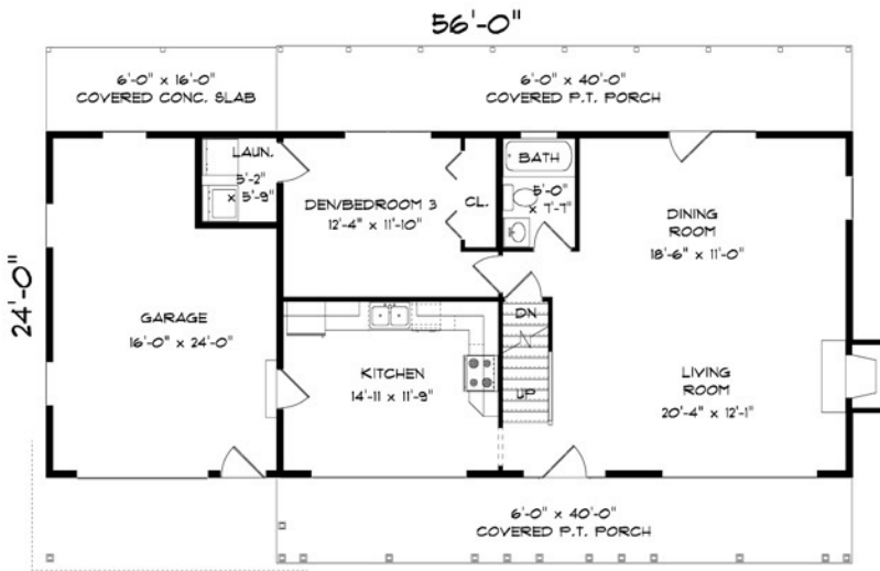
FIRST FLOOR 998 SQUARE FEET
